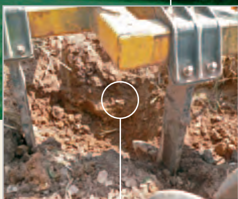
Chisel ploughing in part of the field to remove compacted layer
