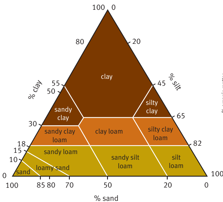
Soil texture classification for mineral soils, and for soils with high organic matter
